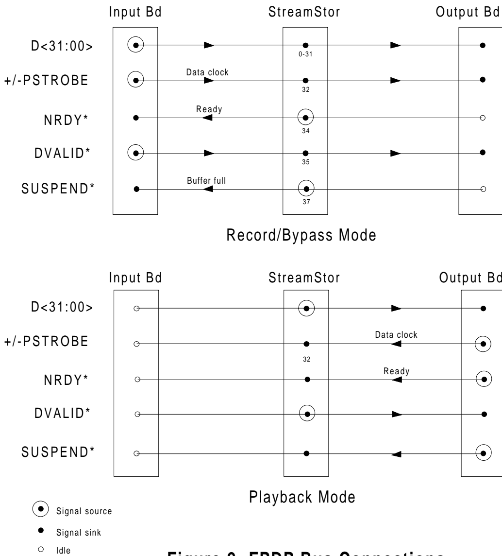
Figure 2: FPDP Bus Connections
