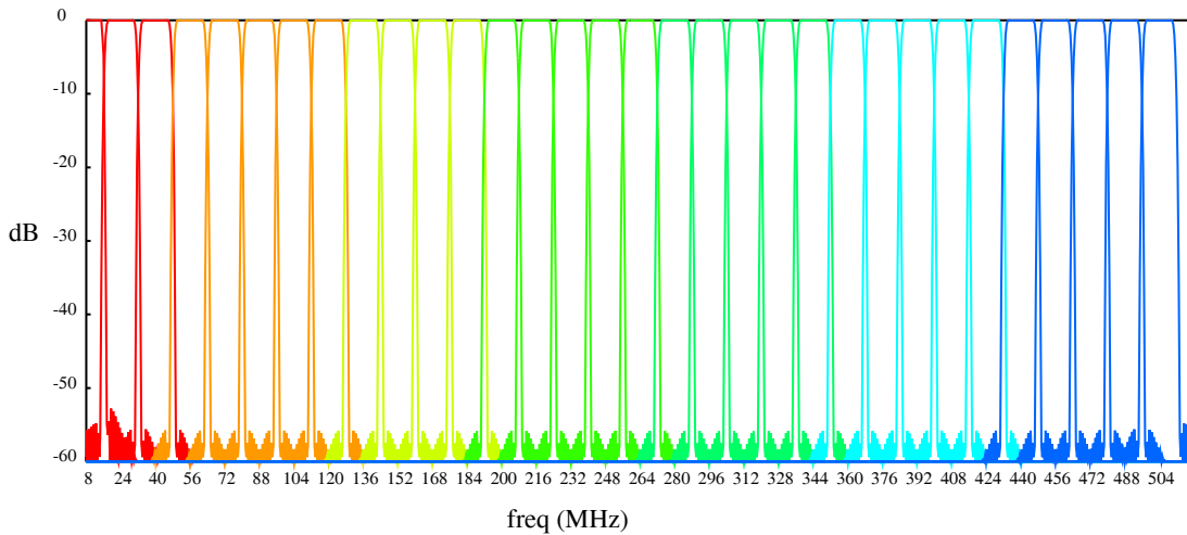
Figure 1. Channel bandpasses from method C
