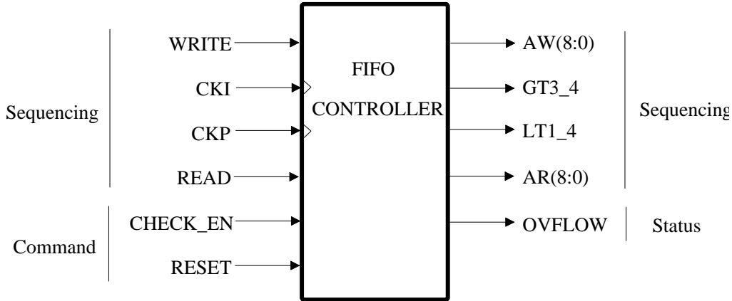
FIGURE 10 FIFO CONTROLLER
