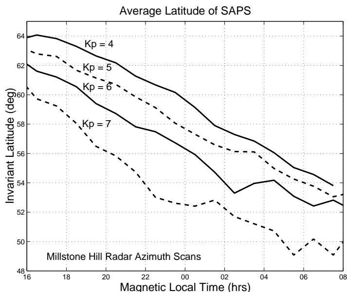
Figure 3. The average latitude of the peak of the polarization stream decreases uniformly as a function of both MLT and increasing K_p index.
