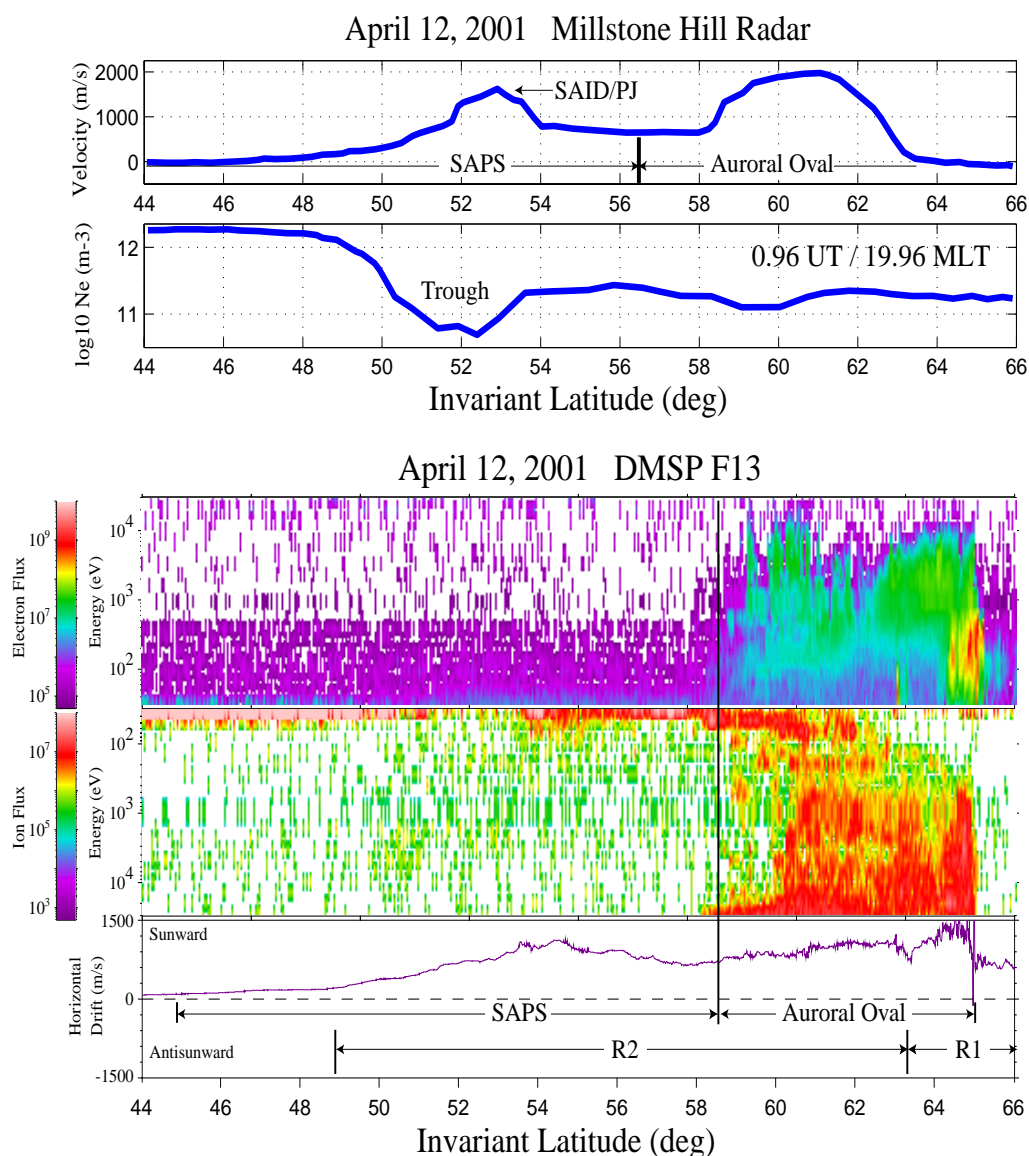
Figure 1. Millstone Hill ISR and simultaneous DMSP pass across the subauroral polarization stream at 20 MLT. SAPS appears as a region of strong westward ion velocity, equatorward of the auroral 2-cell convection and coincident with a deep ionospheric trough. Region 1 (R1) and Region 2 (R2) field aligned currents have been determined using the DMSP magnetometer (not shown). [after Foster and Burke, 2002].
