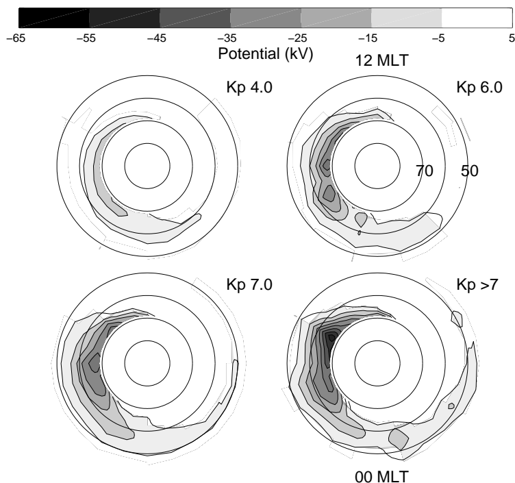
Figure 7. Patterns of negative electrostatic potential have been derived by poleward integration of the average westward velocity across the subauroral region for four levels of the Kp index. Circles are spaced at 10^\circ increments of invariant latitude. Only the region of negative potential is shown in order to emphasize its extent across the night sector between 50^\circ \Lambda and 60^\circ \Lambda . Regions of equatorward-directed potential gradient are associated with SAPS convection. For Kp > 6 , 15 kV to > 30 kV of potential are associated with the SAPS in the post-midnight subauroral ionosphere.
