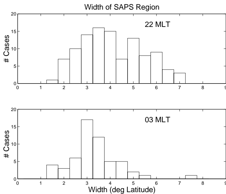
Figure 4. The latitudinal width of the polarization stream determined from the Millstone Hill radar scans is 3^\circ - 5^\circ in the pre-midnight sector and \sim 3^\circ post-midnight.
