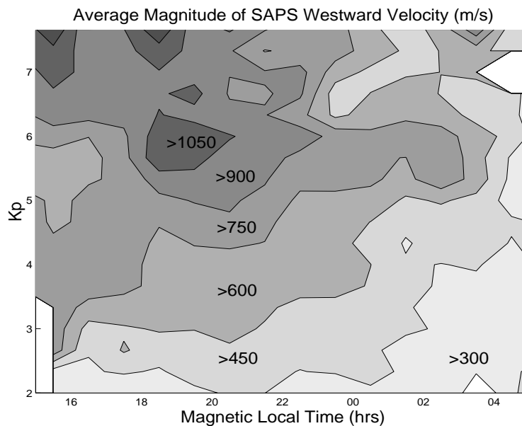
Figure 5. The average magnitude of the peak SAPS westward velocity observed from Millstone Hill has been determined as a function of Kp and MLT. The average SAPS peak velocity exceeds 1000 m/s near 20 MLT for Kp ~ 6 conditions.
