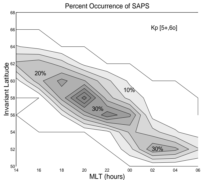
Figure 9. Occurrence probability of SAPS for Kp in the range [5^+, 6^0] exceeds 30% in the pre-midnight sector (19 MLT - 23 MLT) near 57^\circ\Lambda , and in the post-midnight sector near 52^\circ\Lambda .
