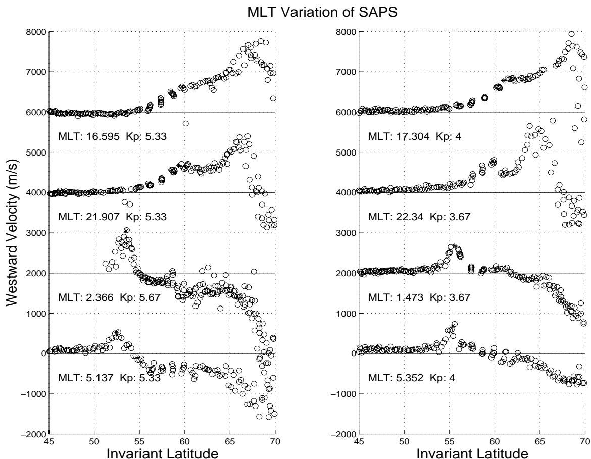
Figure 2. SAPS is seen as an activity-dependent, subauroral westward velocity peak which separates from the high-latitude two-cell convection near dusk and is observed across the midnight sector. Representative individual radar azimuth scans across the SAPS region are shown. Individual radar velocity samples are shown by open circles and our determination of the SAPS peak is indicated by “*”.
